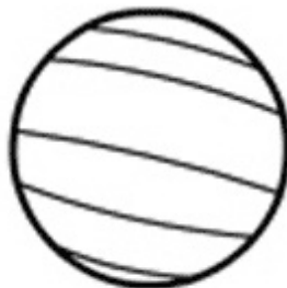
Neptune
