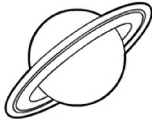
Saturn
